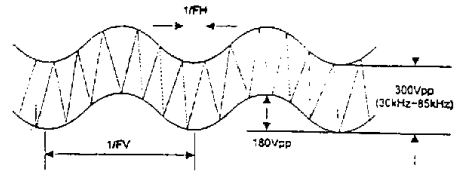
Figure 3-13 Focus Correction Wave
