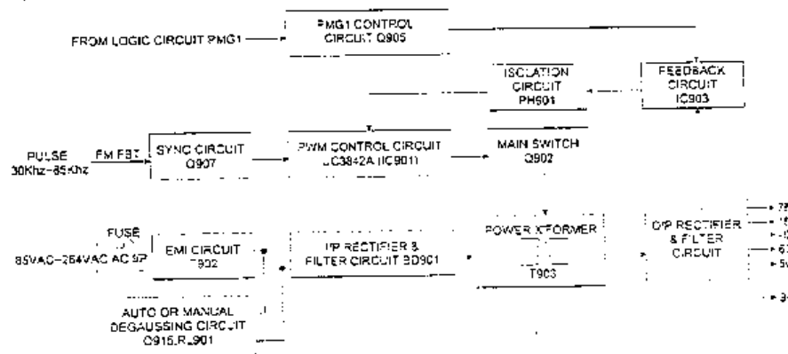
Figure 3-1 Switching Power Supply Block Diagram
