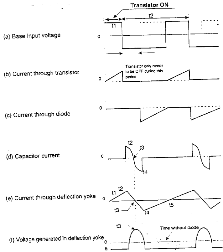
Figure 3-8 Horizontal Output Voltage/Current Waves
