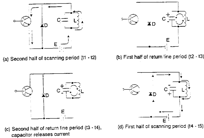
Figure 3-9 Polarity of Transformer Voltage
