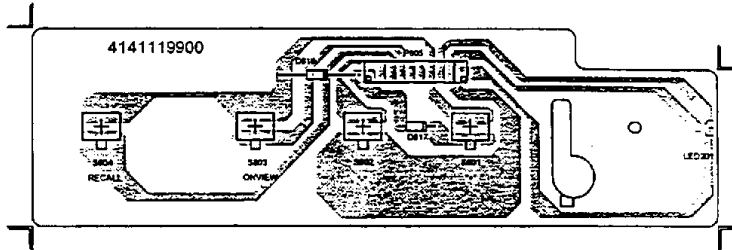
Figure 6-3 Control Board (Solder Side)
