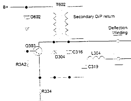
Figure 3-10 Basic Horizontal Deflection Output Circuit
