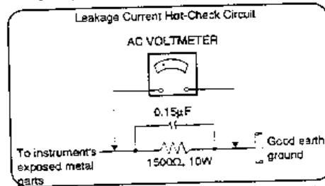
Example of Leakage Current Hot-Check Circuit
