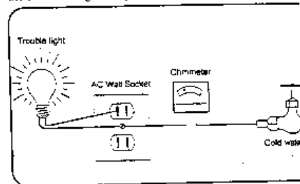
How to Check for Earth Ground
