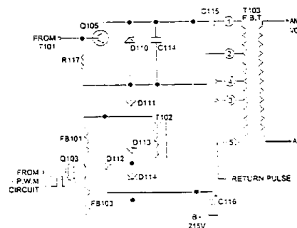
Figure 3-12 Basic High Voltage Output Circuit
