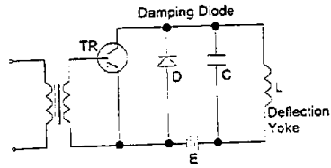
Figure 3-6 The Basic Deflection Circuit
